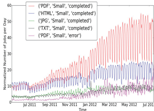
Figure 7. Normalized number of top 5 job types per day (excluding MAFF).
